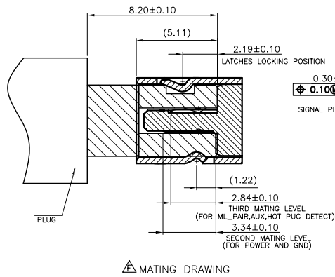
MATING DRAWING
