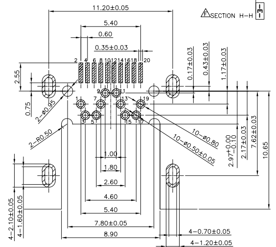
RECOMMENDED PCB LAYOUT(TOP VIEW) (THICKNESS=1.2±0.10mm) (TOLERANCE=±0.05mm)
