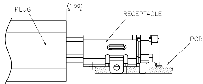
MATING DRAWING
