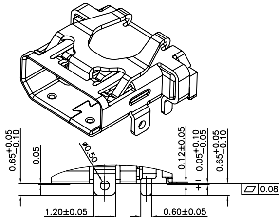
DETAIL "H"
