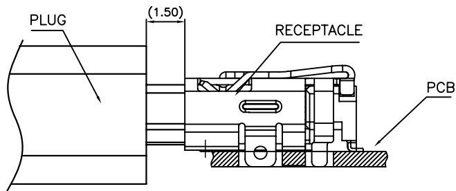
MATING DRAWING
