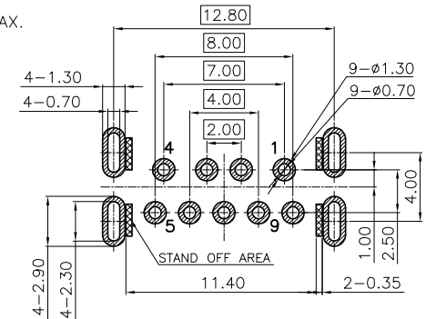
TOLERANCE: ±0.05, THICKNESS: 1.56mm RECOMMENDED PCB LAYOUT (TOP VIEW)
