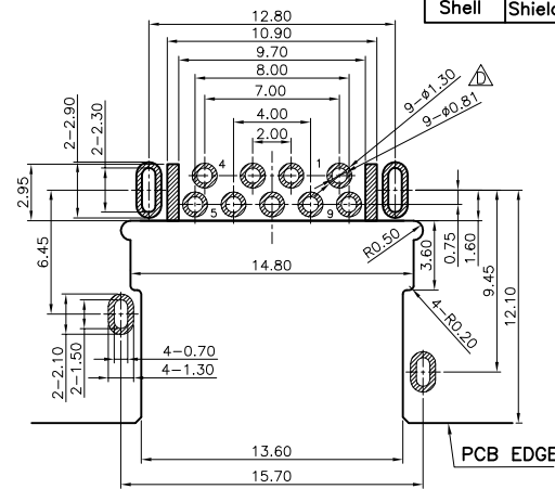
RECOMMENDED PCB LAYOUT(TOP VIEW) (DEFAULT DIMENSION TOL=±0.03mm) (THICKNESS=1.20±0.05mm)
