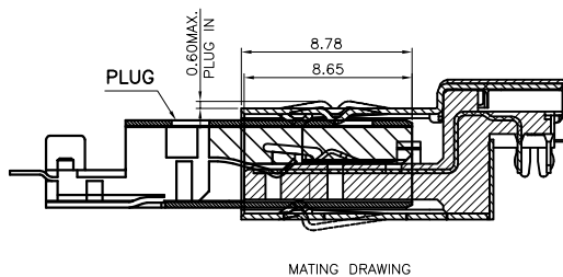
MATING DRAWING
