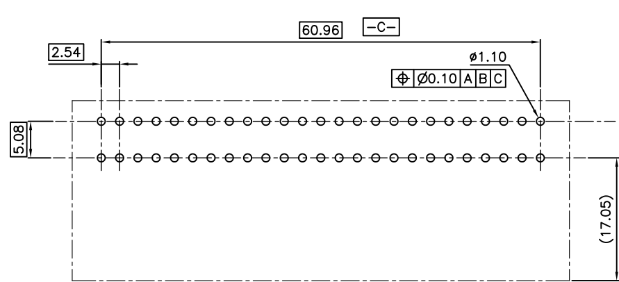
RECOMMENDED PCB LAYOUT (TOLERANCE \pm 0.05 ) (TOP VIEW)
