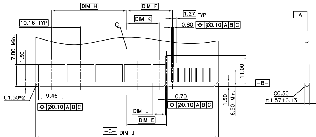
RECOMMENDED EDGE CARD LAYOUT (TOLERANCE ± 0.05)
