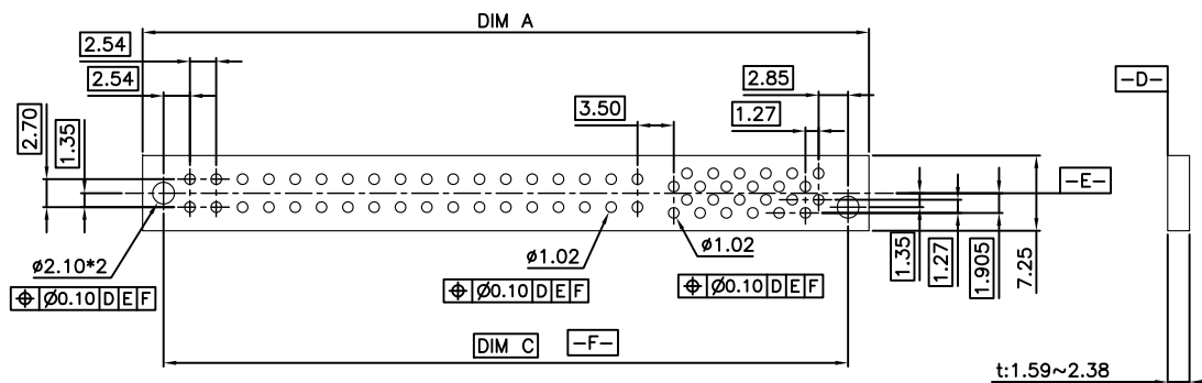
RECOMMENDED PCB LAYOUT (TOP VIEW) (TOLERANCE ± 0.05)
